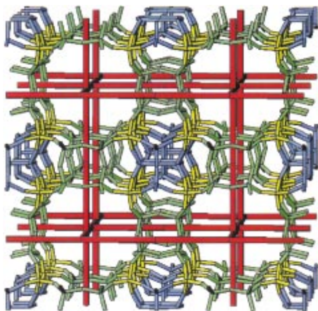
Figure 3. A [001] perspective view of the crystal structure of the calcined polymorph C of zeolite Beta showing the three-dimensional pore system formed by linear channels of nearly circular 12-membered rings intersecting at different heights as indicated by the bars. The pore diameter of the channels calculated from the crystallographic data ranges from 6.3 to 6.6 Å, which is very close to the experimental value of 6.9 Å calculated from the Ar adsorption isotherm by using the Horvath–Kawazoe formalism.
